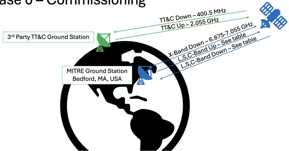
Figure 1: Phase 0 – Commissioning
