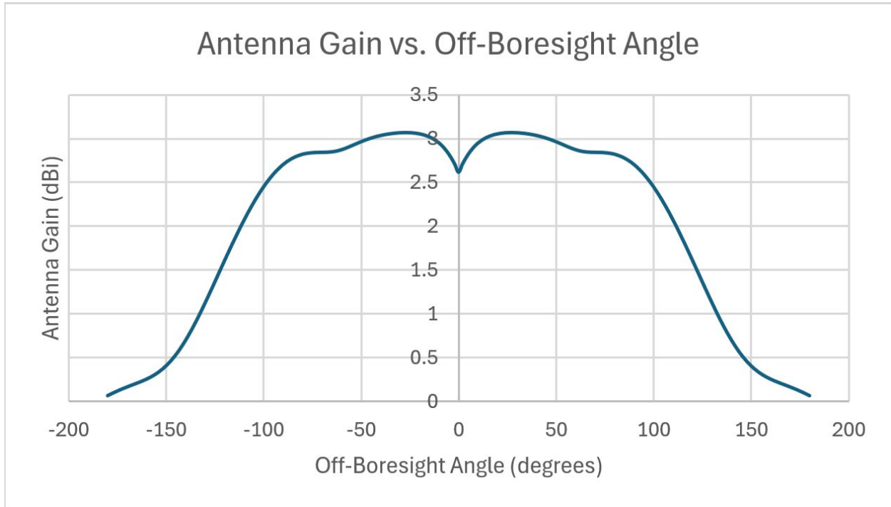
Figure 5 UHF space-Earth and Earth-space Antenna Pattern (TT&C)
