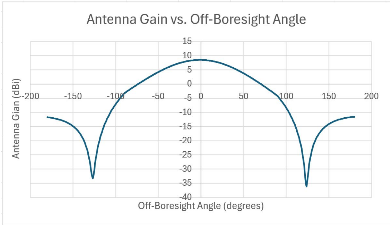
Figure 1 S-band Earth-space Antenna Pattern (1980-2010 MHz MSS) Payload
