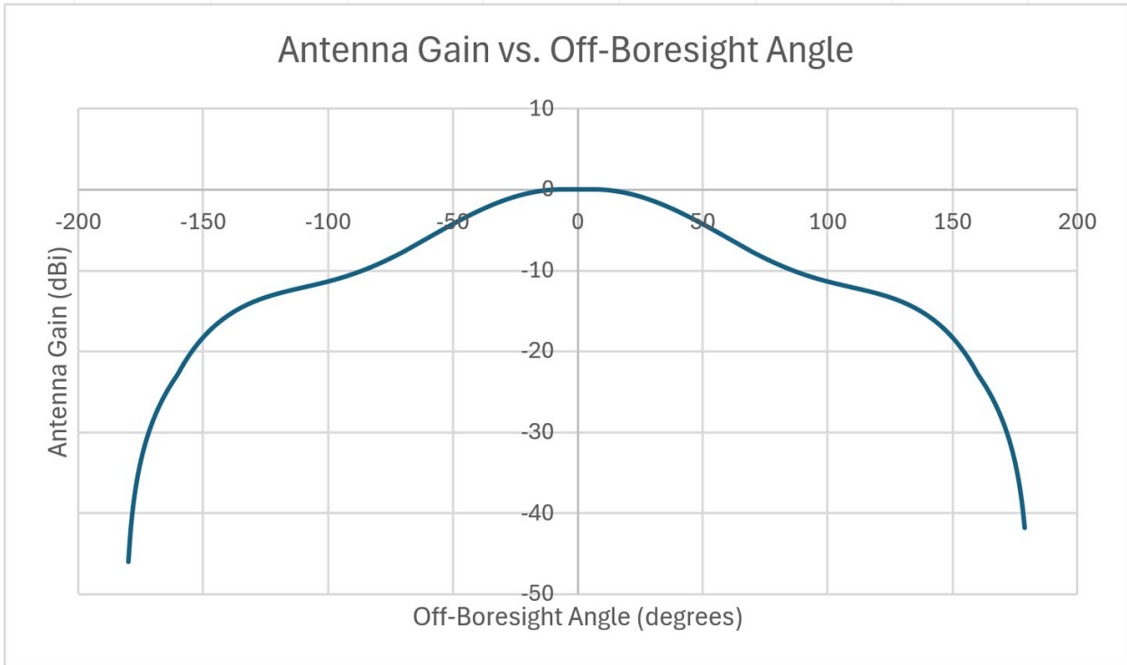
Figure 4 S-band space-Earth Antenna Pattern (2200-2290 MHz) TT&C
