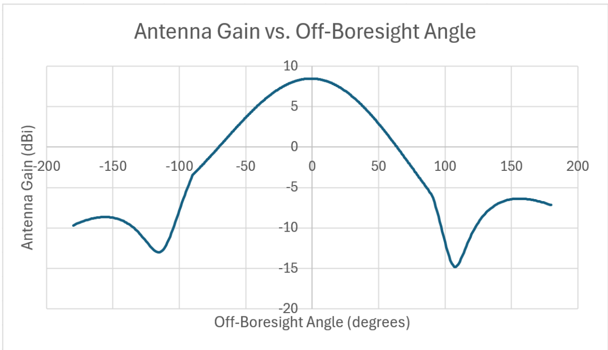
Figure 2 S-band space-Earth Antenna Pattern (2170-2200 MHz MSS) Payload
