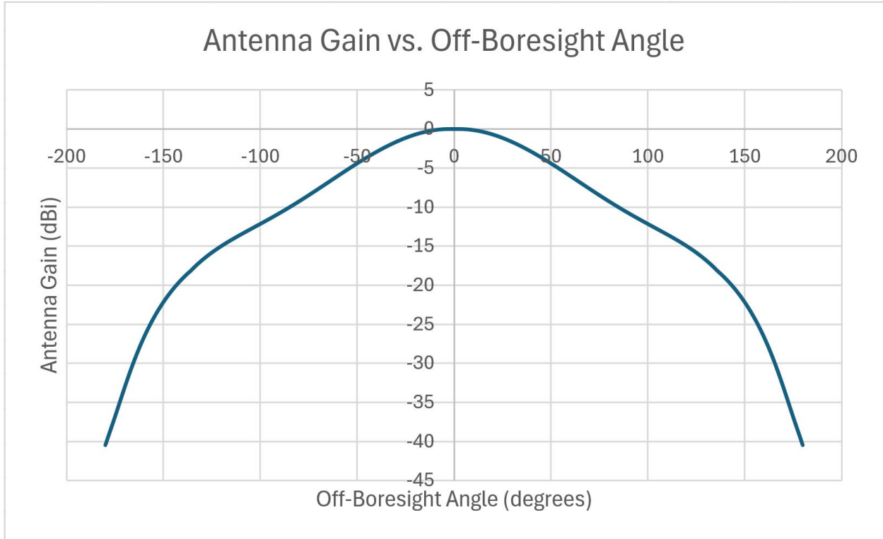
Figure 3 S-band Earth-space Antenna Pattern (2025-2110 MHz) TT&C
