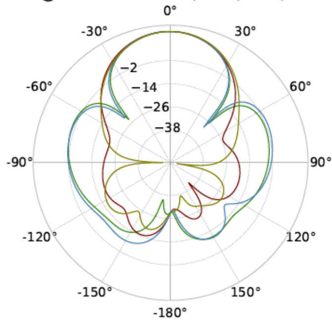
Figure 4: Simulated Radiation Pattern
