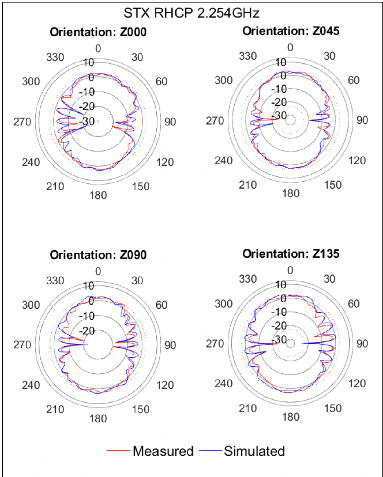
Figure 4: SFL-GNB-COM-SPA Antenna Pattern
