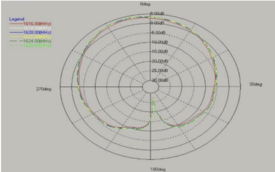
Figure 3: Iridium Antenna Pattern
