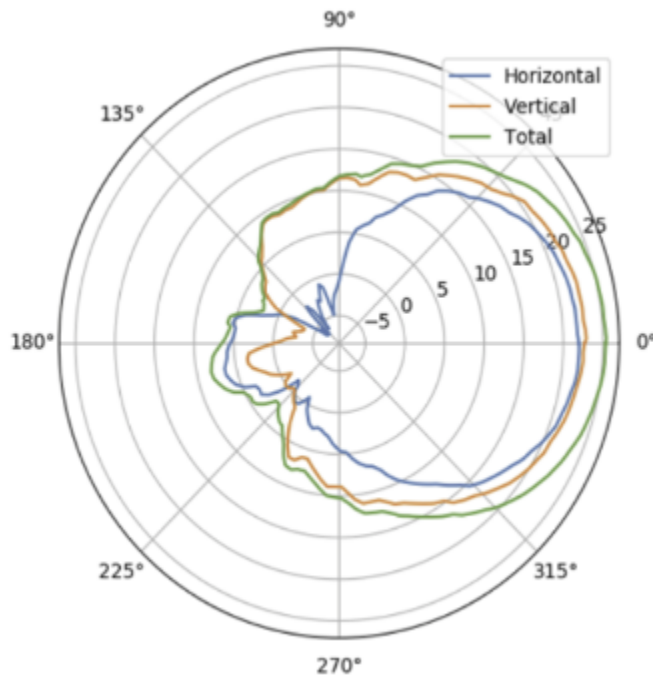
Figure 2: S-band Rx Antenna Pattern
