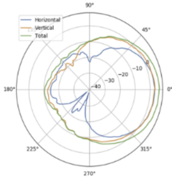
Figure 1: S-band TX Antenna Pattern
