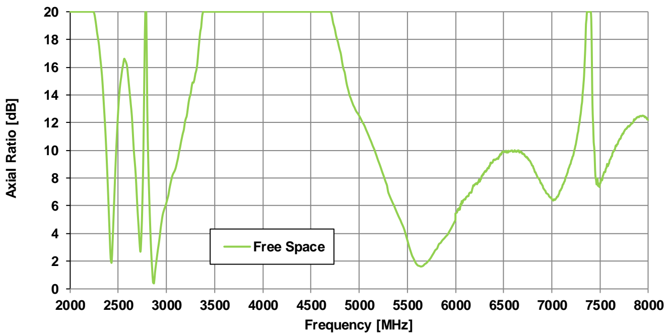
Axial Ratio vs Frequency
