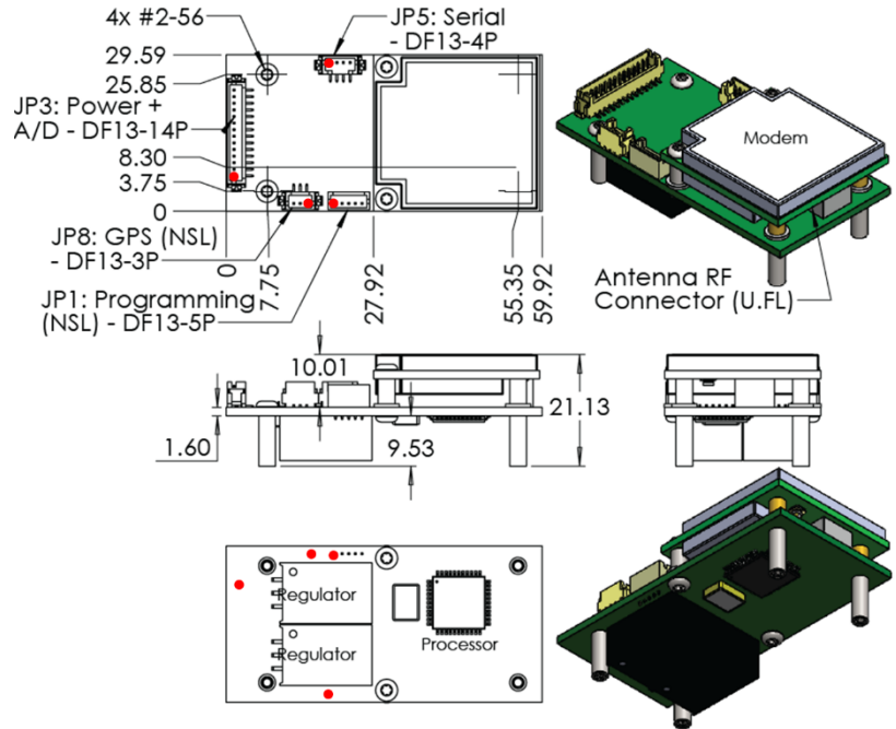
Figure 2 EyeStar-S4 Mechanical Drawing with connectors.
