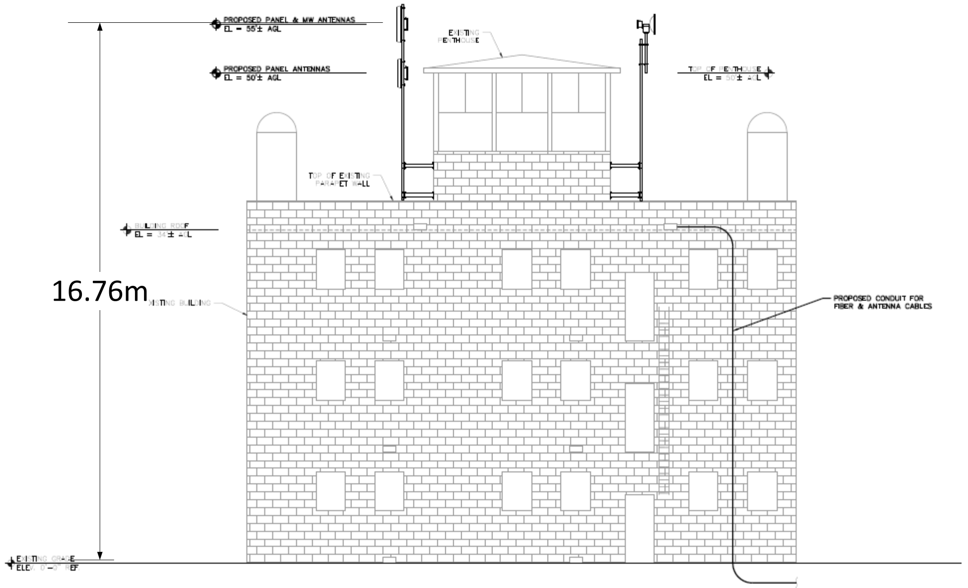
BUILDING ELEVATION
