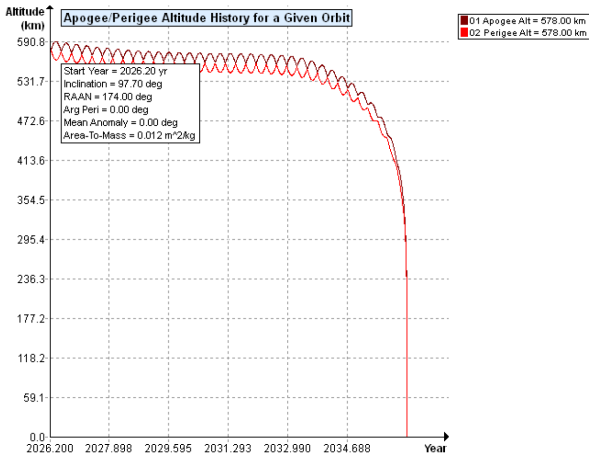
Figure 6-1: Orbit Lifetime
