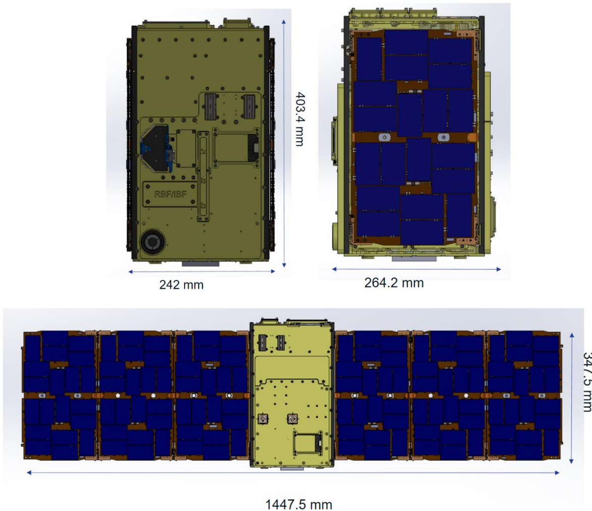
Figure 2-1: Spacecraft Vehicle Layout
