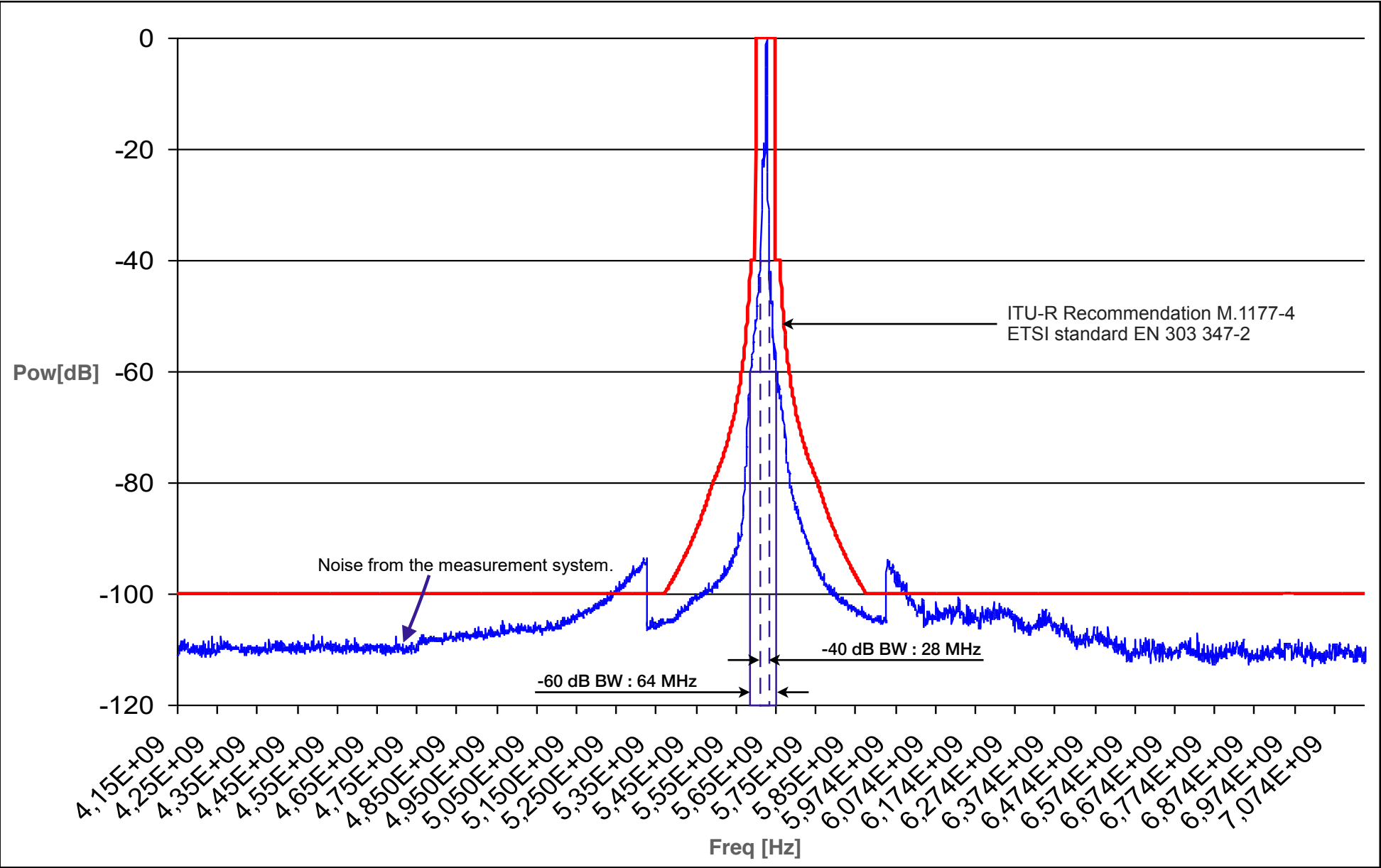
WRM200 Transmitter Spectrum (1 us pulse)
