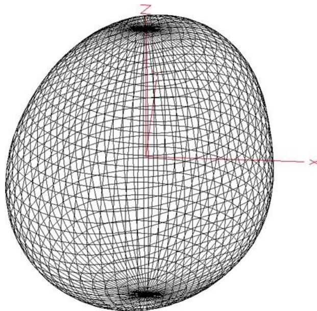
Figure 2: Tyvak-XXXX L-Dipole UHF Antenna Gain Plot
