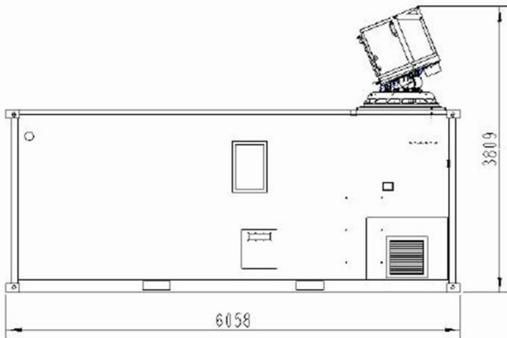
Exhibit No. 2 Antenna Drawing
