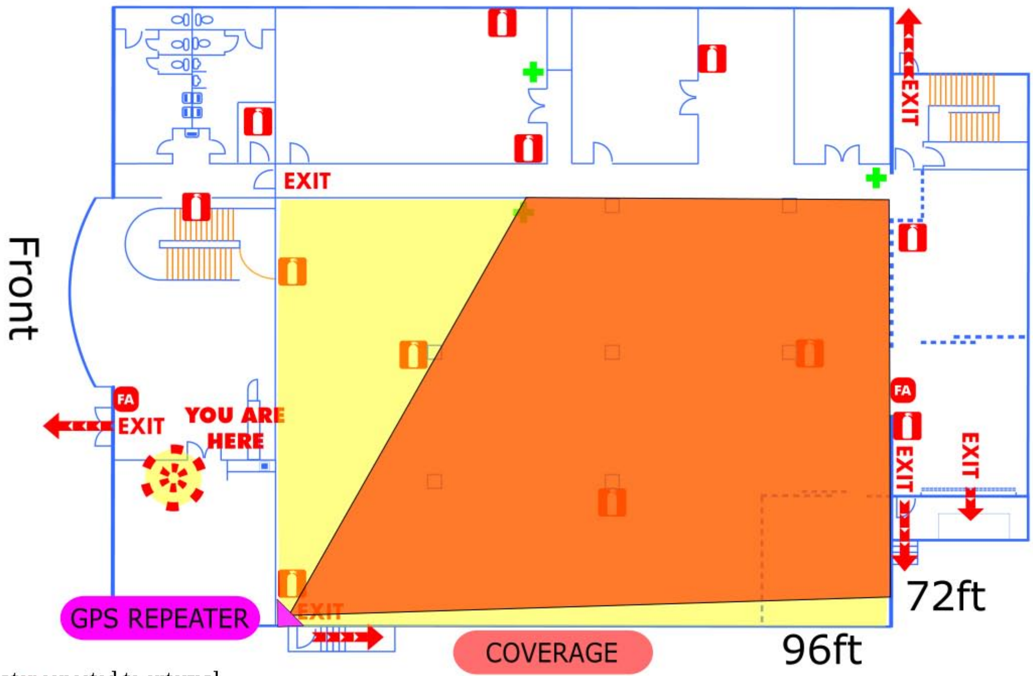
Repeater connected to external antenna via 100 ft. LMR-240
