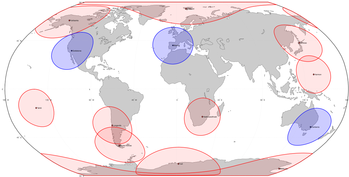
Figure 2.4-2. Transmission footprints for the possible ground stations for GNOMES-1 (in red) and their overlap with DSN station (in blue).
