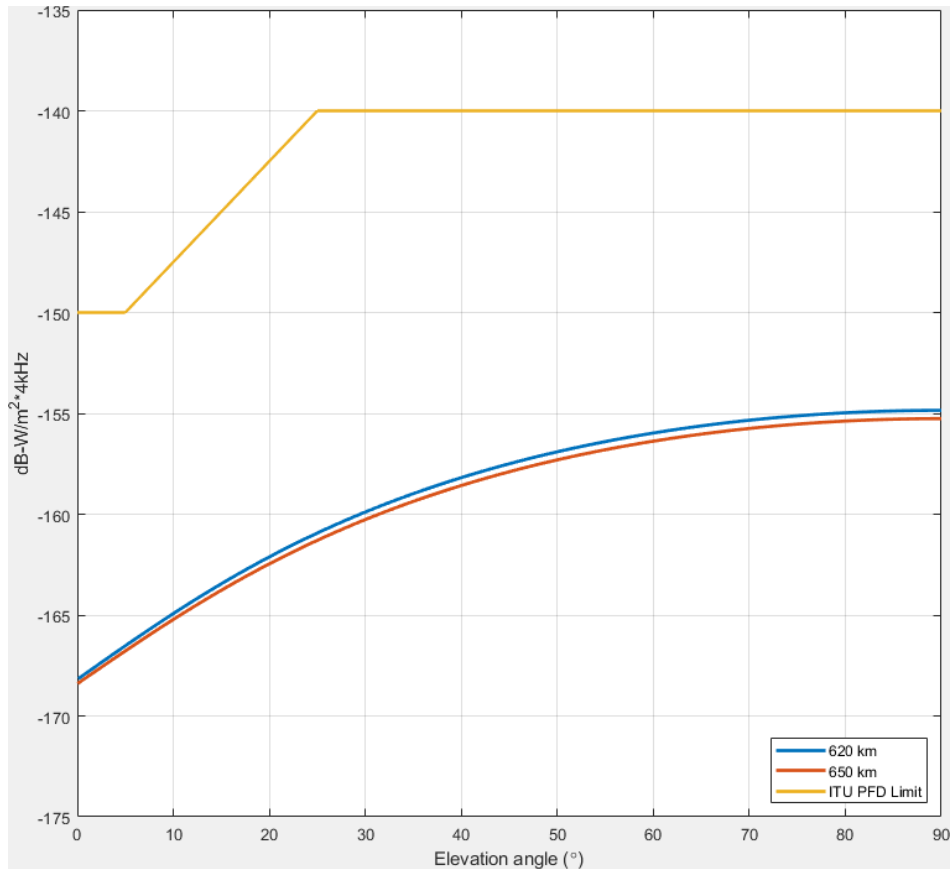
Figure 2.4-1. PFD at the Earth’s surface produced by the X-band downlink radio for GNOMES-1 at the injection and operational altitudes.
