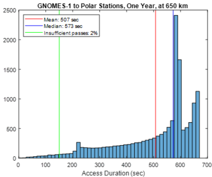
Figure 2.4-3. Pass lengths for GNOMES-1 at 650 km sun-synchronous orbit.
