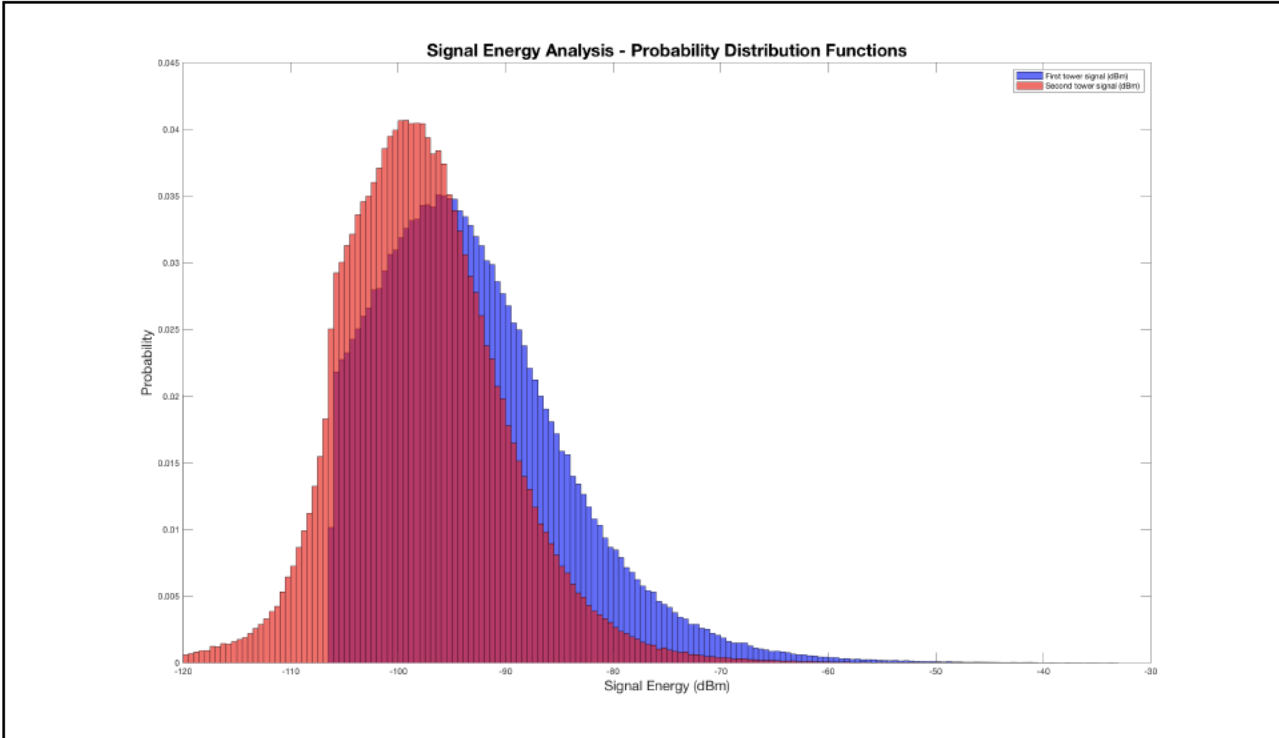
Figure 18 - Probability distribution function (PDF) of the signal energy from the nearest and second nearest tower to any location in the US per the Monte Carlo simulation model
