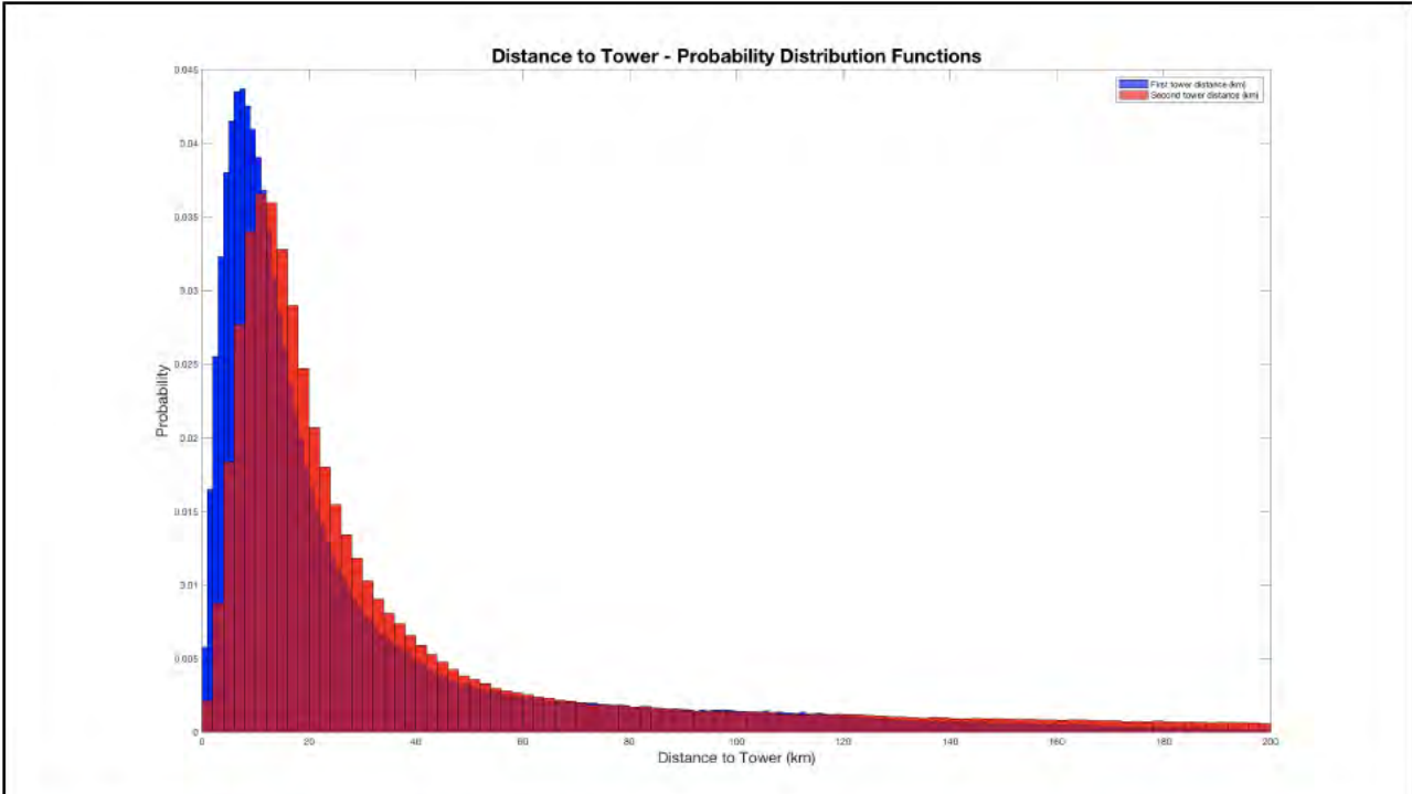
Figure 19 - Probability distribution function (PDF) of the distance to the first and second nearest tower for any location in the US per the Monte Carlo simulation model
