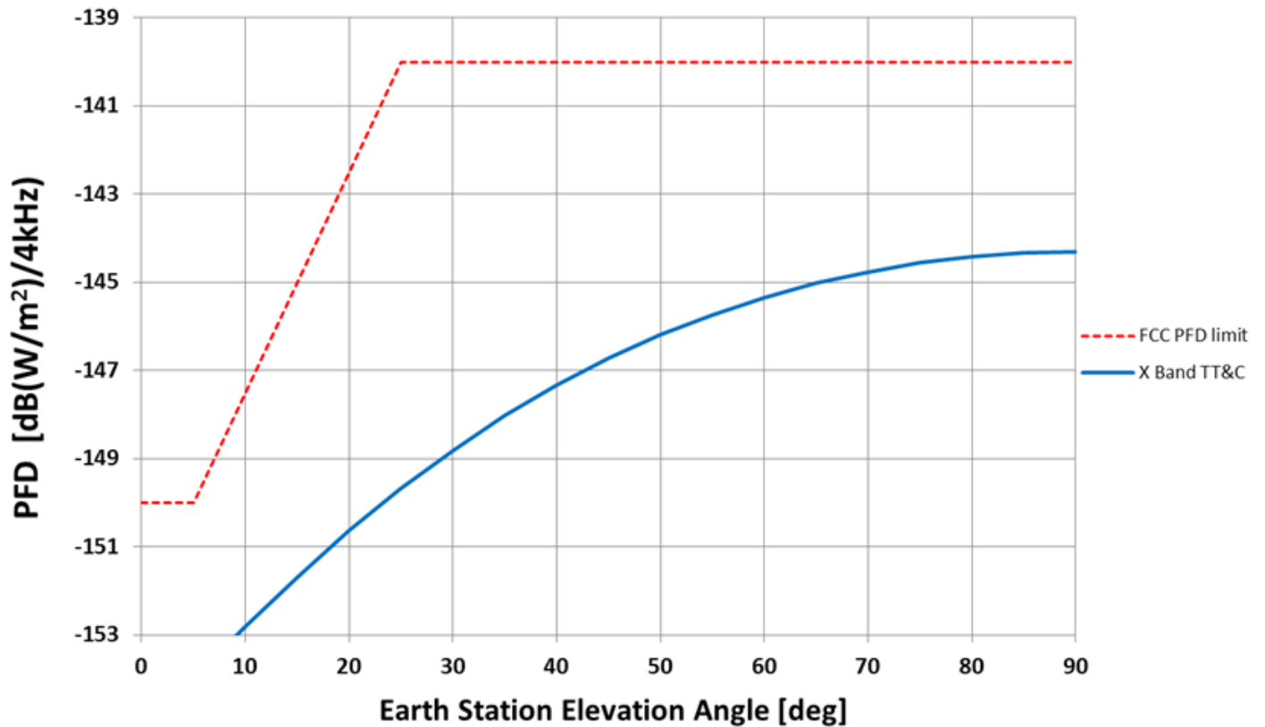
Figure 6. PFD at the surface of the Earth produced by the satellite telemetry downlinks when at 1125 km
