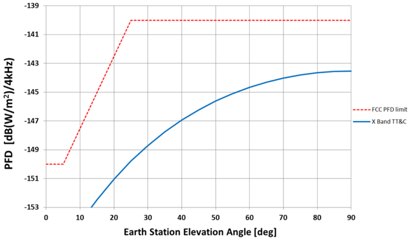
Figure 7. PFD at the surface of the Earth produced by the satellite telemetry downlinks when at 514 km
