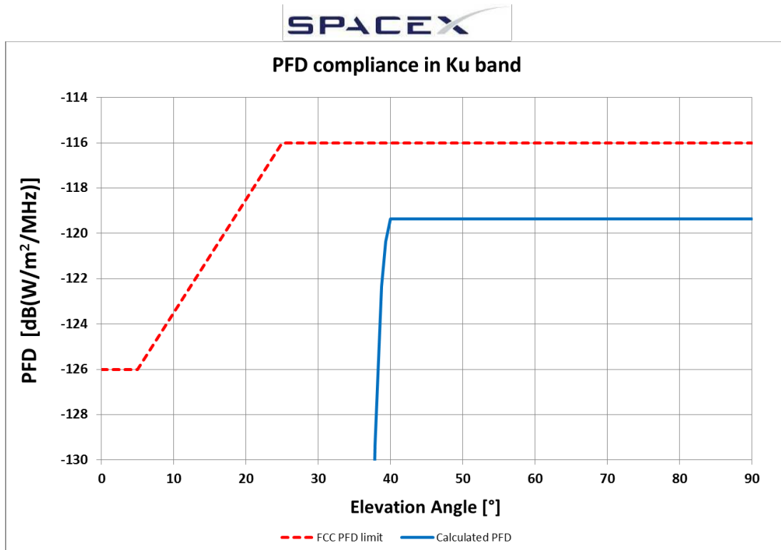
Figure 2. PFD at the surface of the Earth produced by the Ku band downlink transmissions versus elevation angle (1125 km orbit).
