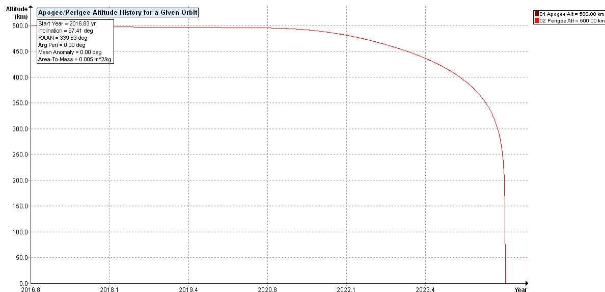
Figure 6: RANGE orbit history for low-drag configuration
