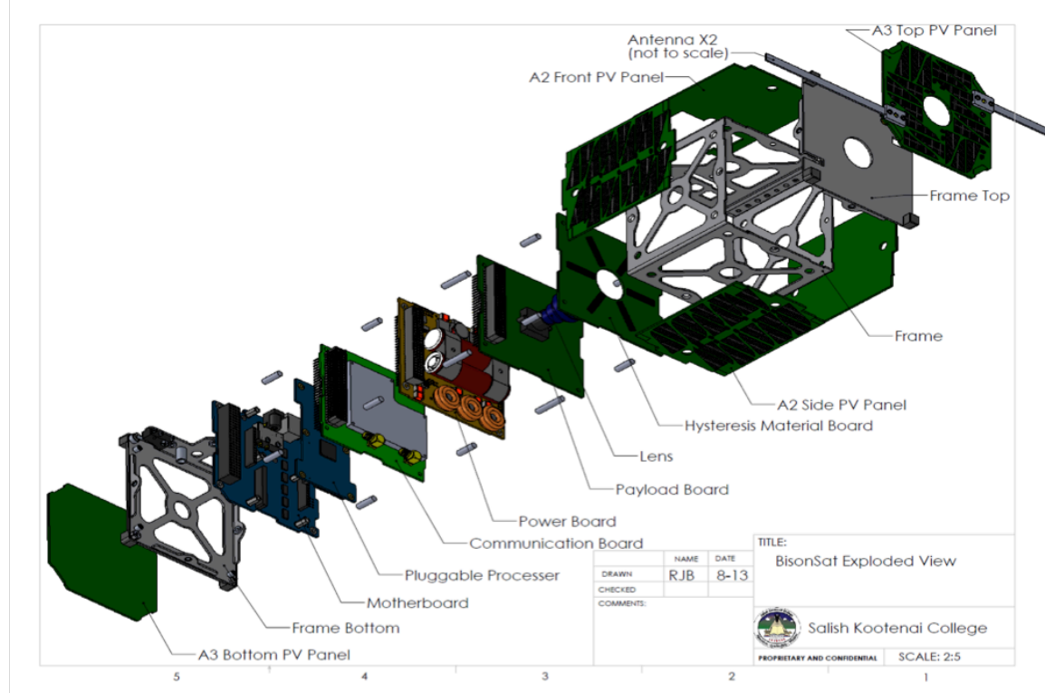
Figure 2: BisonSat Expanded View
