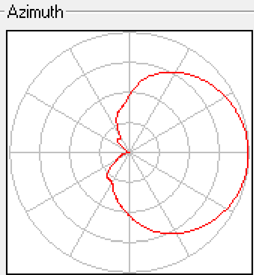
Azimuth Beamwidth: 66.3°
