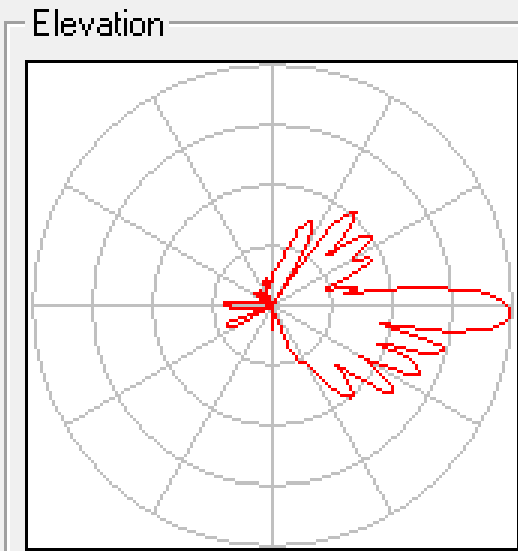
Elevation Beamwidth: 7.9°
