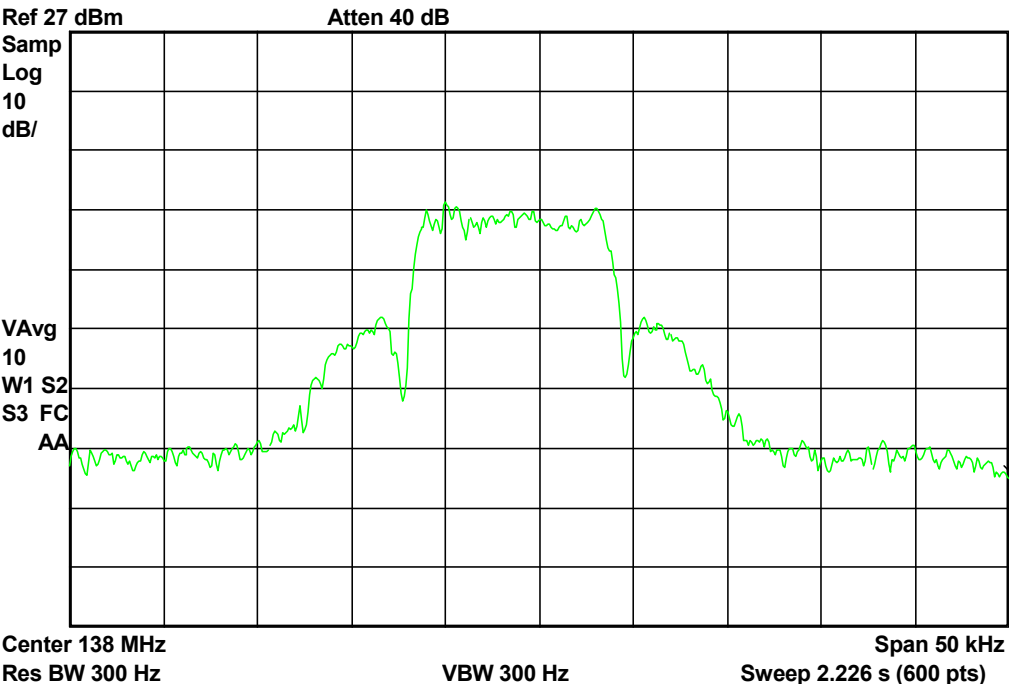
Lithium – 1 GFSK 9600 Baud Output Spectrum
