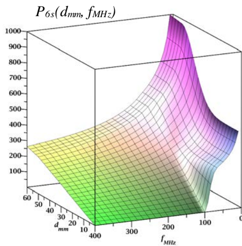
Fig. B.2 – Smoothed function P_{6S}(d_{mm}, f_{MHz}) (left), vs. the original definition of P_6 (right)
