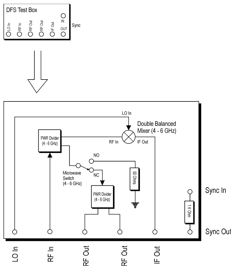
Figure 9c: Example DFS Test Box
