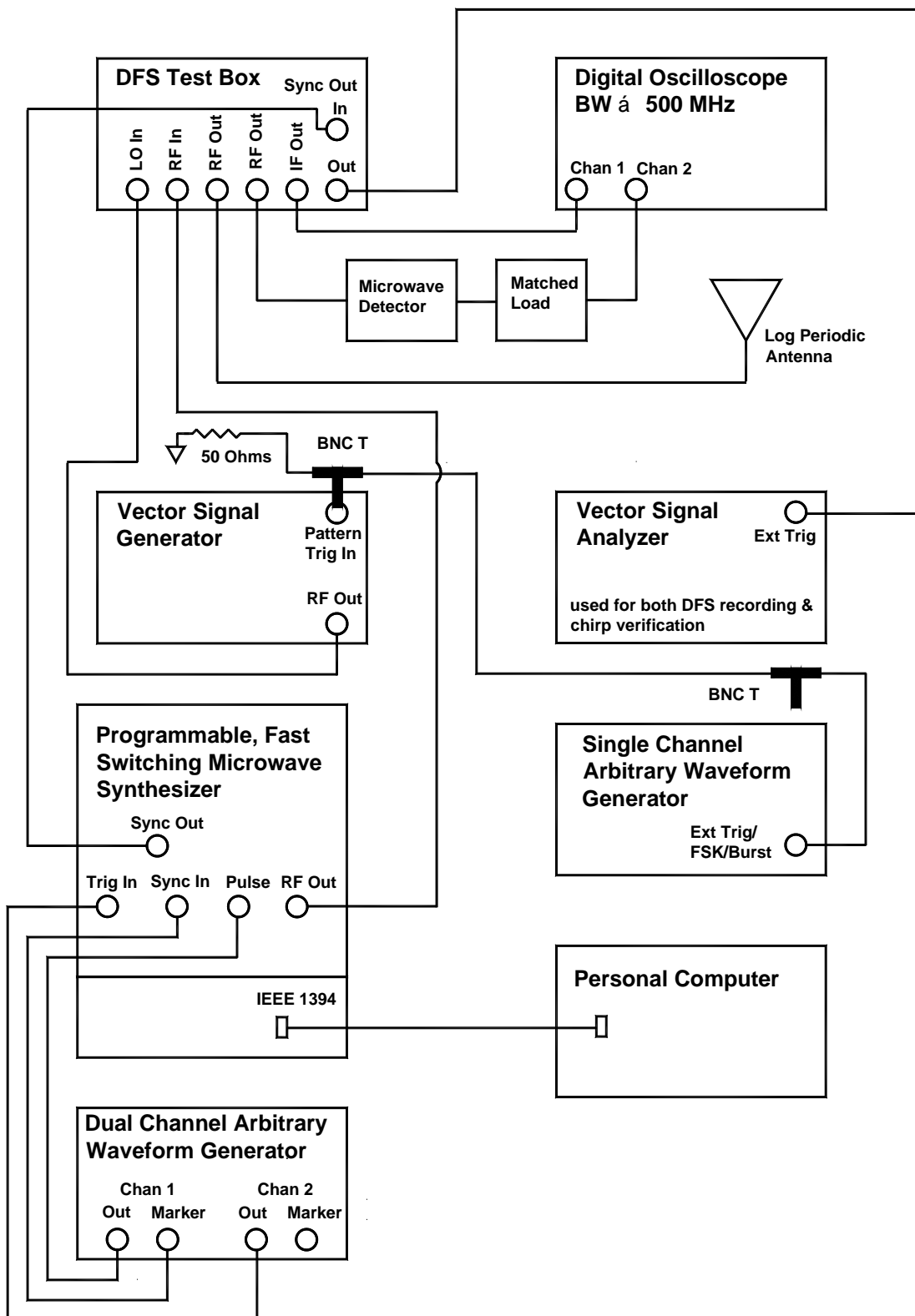
Figure 9b: Example Frequency Hopping Radar Waveform Generator
