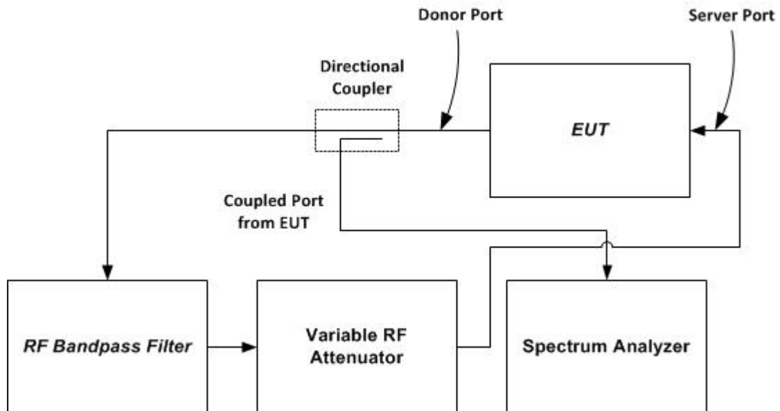
Figure 8 – Oscillation detection instrumentation test setup
