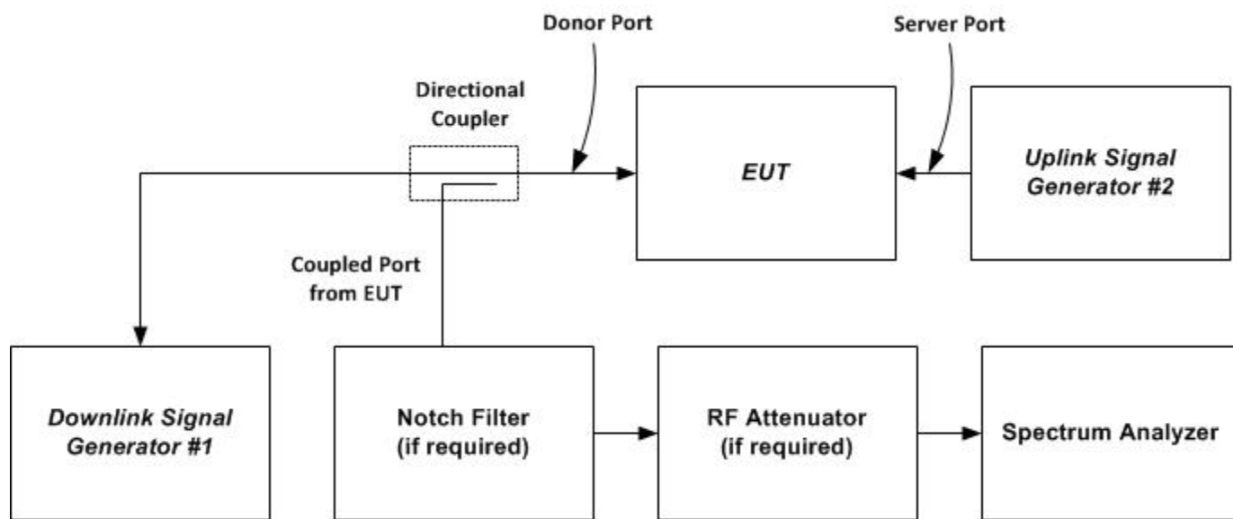
Figure 6 – Variable gain instrumentation test setup
