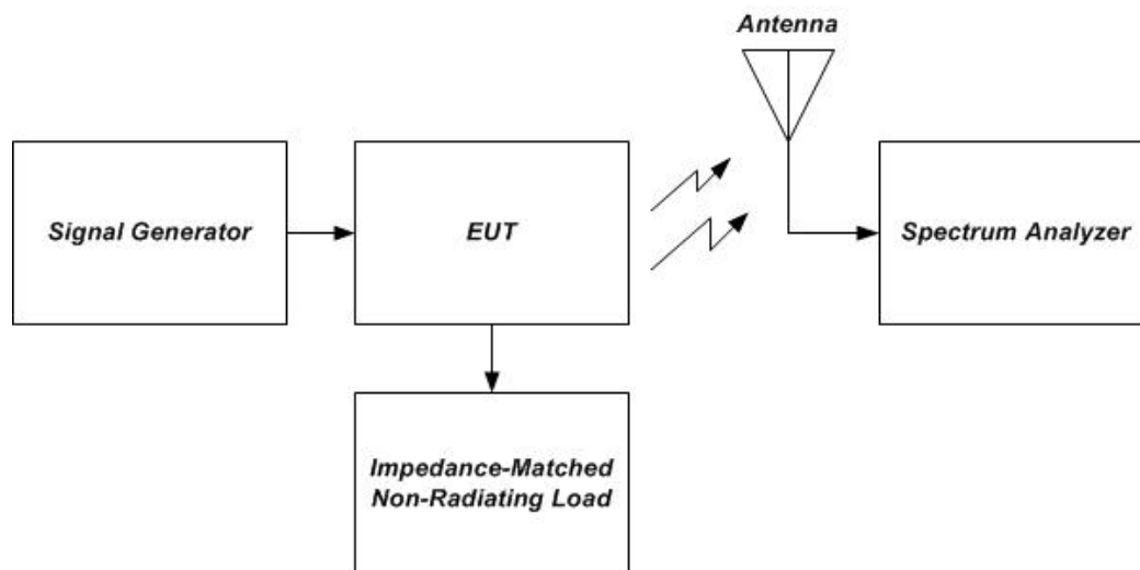
Figure 9 – Radiated spurious emissions test instrumentation setup
