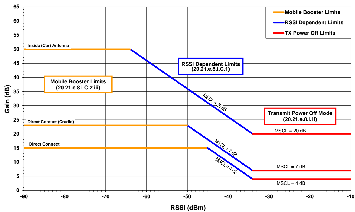
Figure D-3. Mobile Wideband Consumer Signal Booster Variable Gain Limits.
