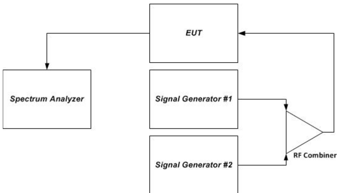
Figure 2 – Intermodulation product instrumentation test setup
