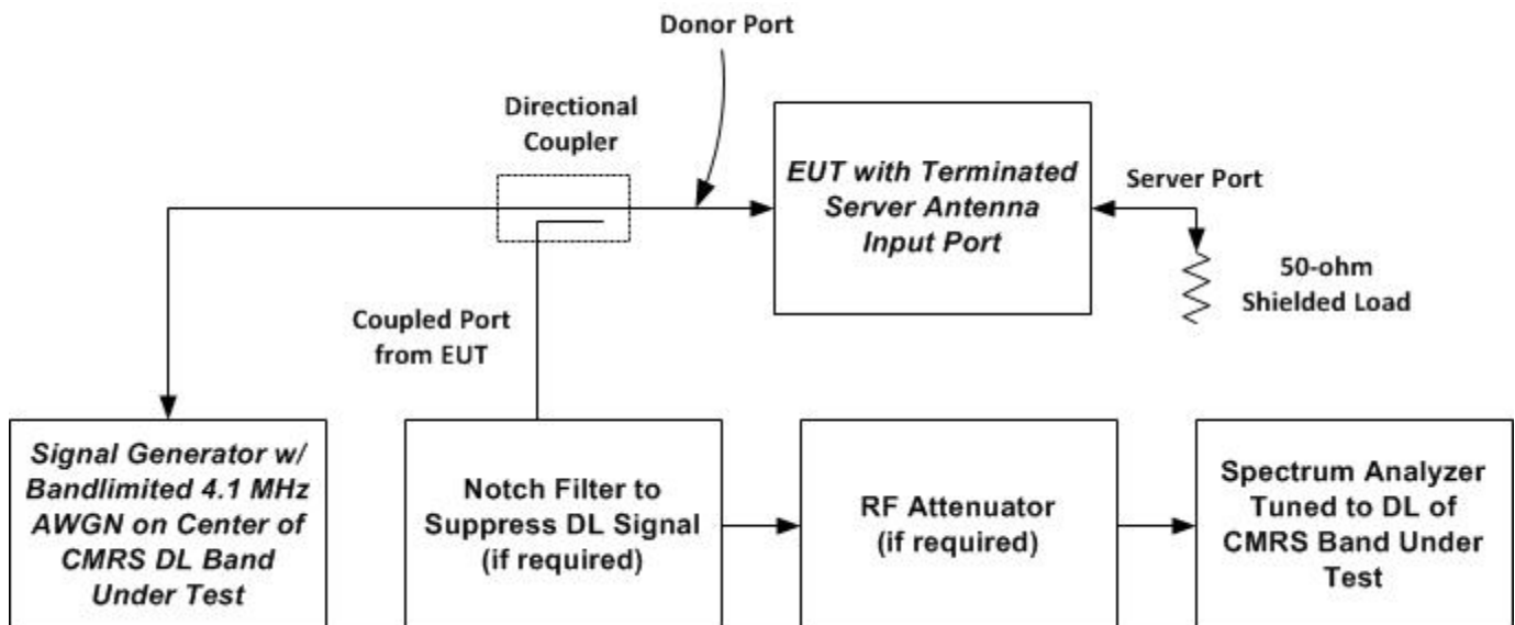
Figure 5 – Test setup downlink noise power measurement in the presence of a downlink signal
